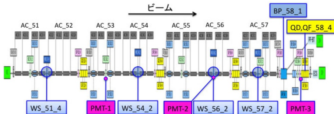
Figure 10: Layout of wire scanner system at 5 sector.
