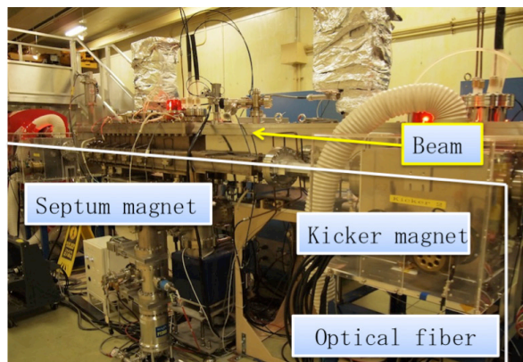
Figure 4: The photograph of PF injection septum magnet.
