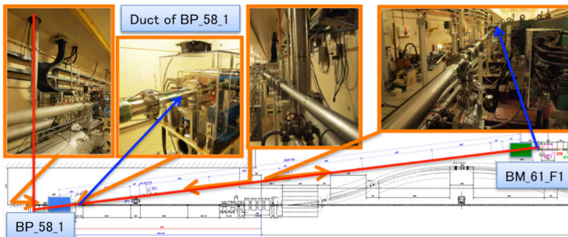
Figure 2: Layout of the PF beam line at the third switching yard.
