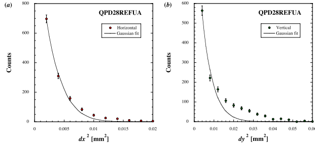
Figure 4: Distribution plots of (a) the x and (b) y square residuals based on the linear-regression analysis in the time traces of the displacements of QPD28REFUA. The solid lines are Gaussian-function fits of the data.
