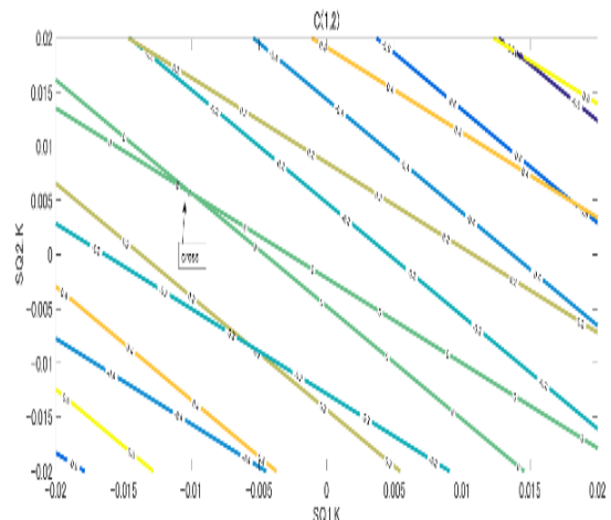
Figure 2: Contour maps of C_{12} .
