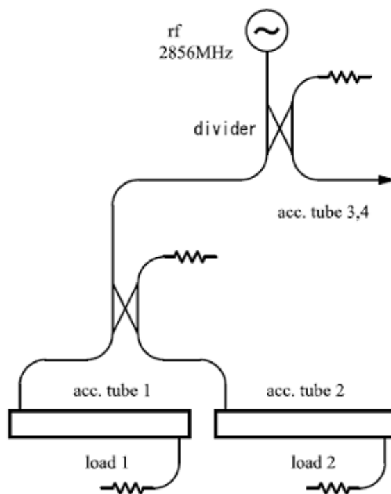
Figure 1: Structure of acceleration unit.
