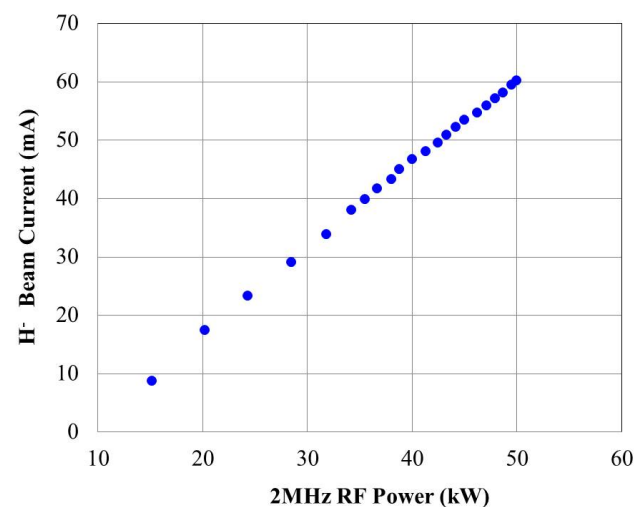
Figure 7: Relation between 2MHz RF power and H- beam current from an RF ion source with a J-PARC antenna.
