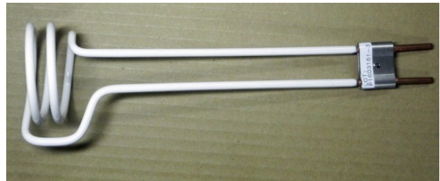
Figure 6: Photograph of a J-PARC antenna.
