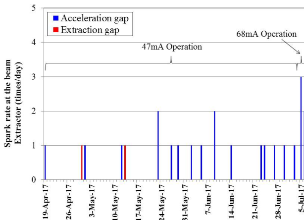
Figure 4: Spark rate at the beam extractor of the source during RUN#75.
