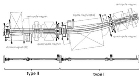
Figure 2: Beam ducts for the arc sections.
