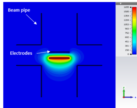
Figure 6: Potential contours on the cross section of the chopper's electrodes and beam pipe.
