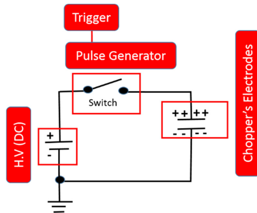
Figure 7: Electrical design of the chopper system.
