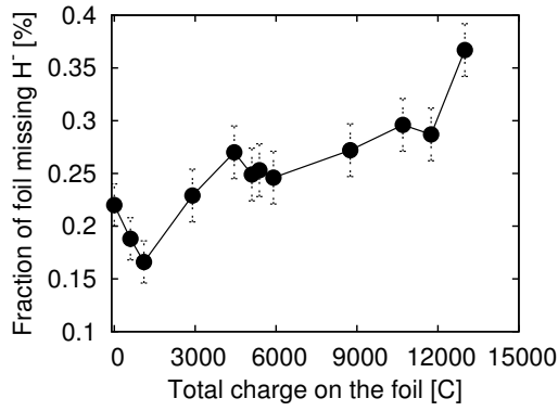
Figure 2: Measured unstripped H - as a function of charge via the foil during beam operation. The missing H - was increased nearly 3 times higher as compared to that in the beginning of the operation. Such an increase of the waste beam may limits the foil lifetime at 1 MW operation.
