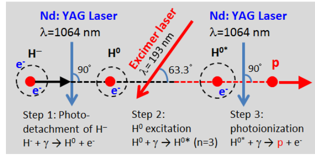
Figure 3: Schematic view of principle for H - stripping to proton by using only lasers. Noted parameters are typical ones estimated for the 400 MeV H - beam energy.
