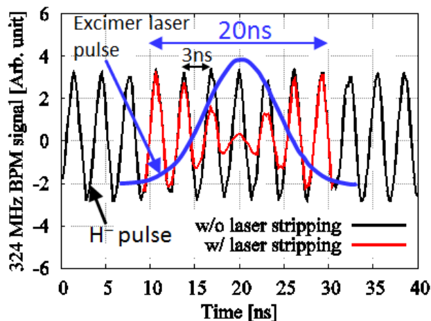
Figure 5: A typical 324 MHz H^- micro pulse structure measured by BPM pickup (black). The blue curve is a given laser pulse by which the H^- is expected to be stripped to protons as shown by the red curve.
