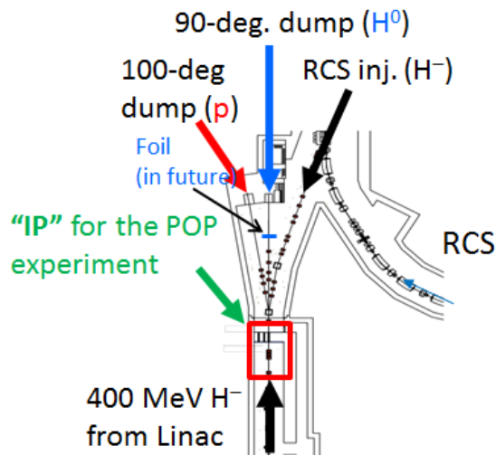
Figure 4: A schematic view of the end section J-PARC L-3BT. The H^- laser stripping POP experimental devices will be installed in the place as shown by red rectangular box. We can simultaneously measure all three charge fractions in the downstream. Namely, fully stripped protons, neutral H^0 (by further stripping) and the unstripped H^- can be measured in the 100-deg. dump, 90-deg. dump, and the RCS injection line, respectively.
