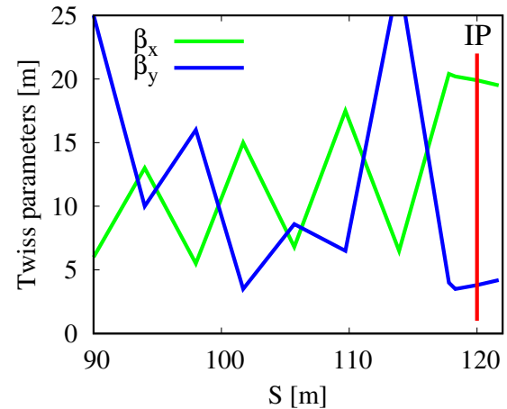
Figure 8: Measurement results of 1st trail of \beta_x and \beta_y optimization for the POP experiment. The measured values at the IP are already very close to expected values, but \beta_y needs to be further reduced.
