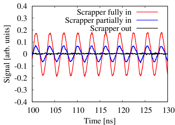
Figure 9: Measured 324 MHz proton beam signal taken by a BPM at the 100-deg. dump. The H^- was stripped to protons by inserting a beam scrapper, placed upstream of the IP.
