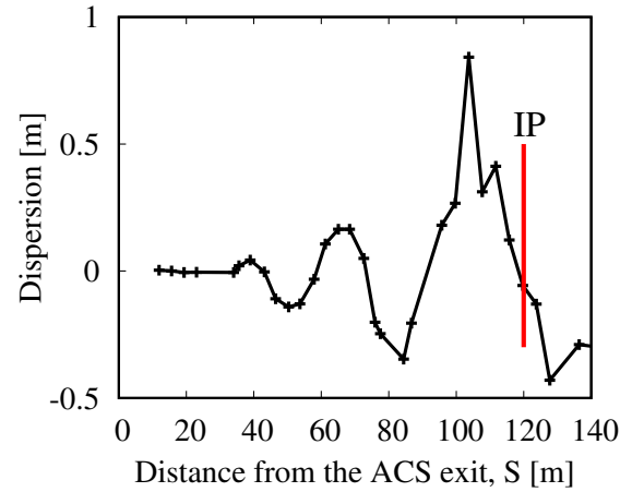
Figure 7: First measurement result of dispersion function optimization of 400 MeV H^- at the IP. The D' at present is obtained to be -0.13 , but further studies will be continued to get the desired value.
