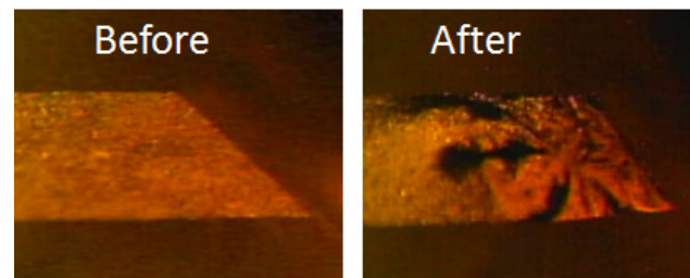
Figure 1: Typical pictures of stripper foil before and after beam irradiation for about 5 month at RCS, but only with 0.3 MW beam power. Deformation of the foil due to beam irradiation caused a rapid increase of the waste beam.
