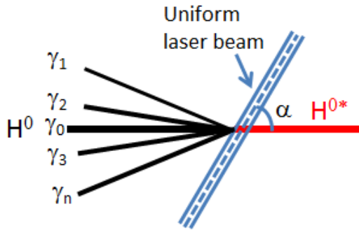
Figure 6: Schematic view of dispersion tailoring method in order to obtain same laser frequency for all hydrogen atoms in their rest frame.
