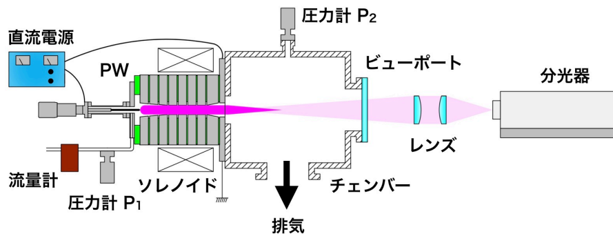
Figure 3: Experimental setup.
