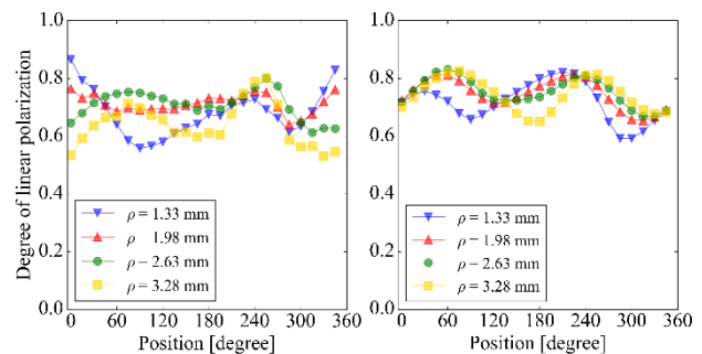
Figure 6: Degree of linear polarization on the observing plane. The left and right figures are measurements and simulation results corresponding to Fig. 4. The horizontal axis and \rho indicate the position as azimuthal angle and distance from center. [5]
