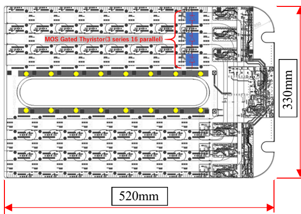
Figure 2: Board appearance.
