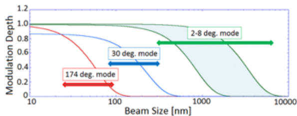
Figure 4: Range of the Beam size measurement, IPBSM.
