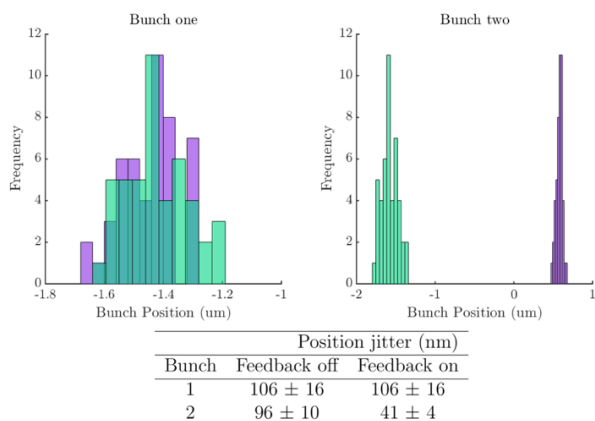
Figure 8: Beam position at IP BPM w/wo FONT.
