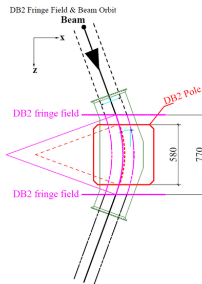
Figure 6: Magnetic length and fringe field.
