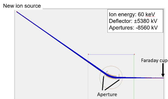
Figure 2: The result of a trajectory simulation of the C_{60} negative ion beams passing.
