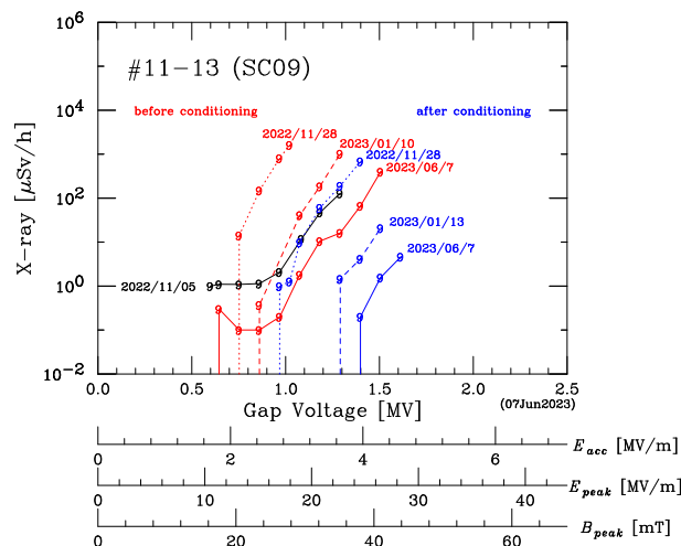
Figure 11: X-ray levels before and after conditioning.
