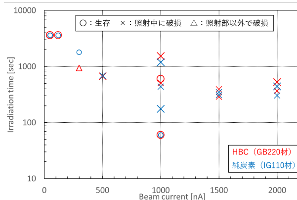
Figure 1: Result of foil durability test against Ar ion irradiation.
