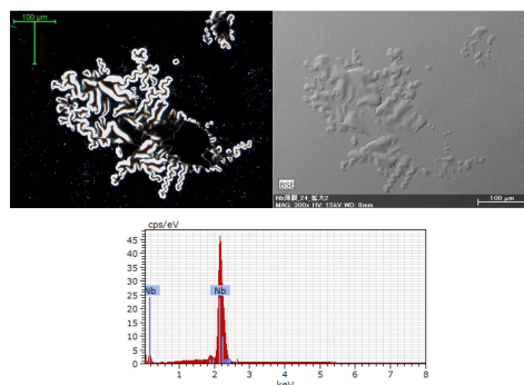
Figure 10: SEM-EDS spectrum on the pit of the Nb coin sample in Fig. 6.
