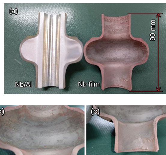
Figure 4: Cross-section of the Nb/Al mandrel similar to 3.9 Hz SRF cavities; (a) as-CSed Nb/Al mandrel and Nb film alone dissolved by HCl solution, magnified pictures of (b) equator part, and (c) iris part.
