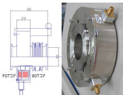
Figure 2: Layout of current transformer (SCT and FCT).
