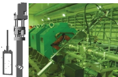
Figure 4: Layout of wire scanner monitor.
