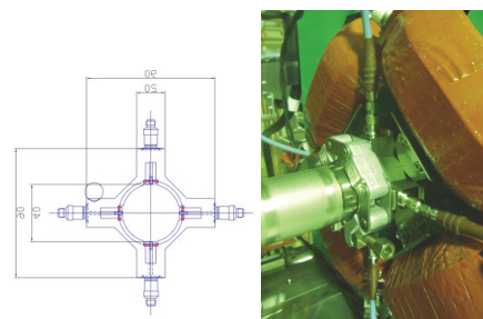
Figure 3: Layout of beam position monitor.
