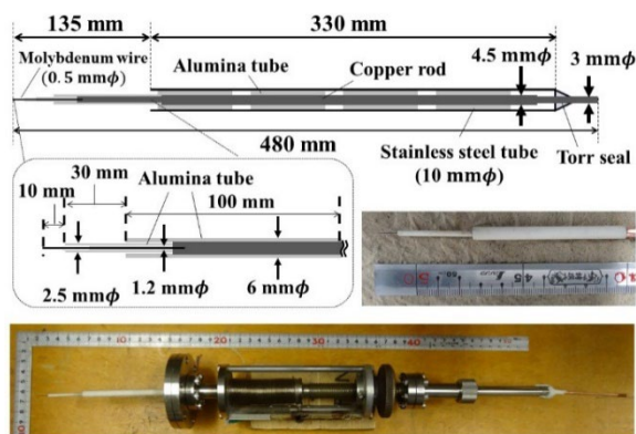
Figure 6: Langmuir probe 1, 2 (LP1, LP2).
