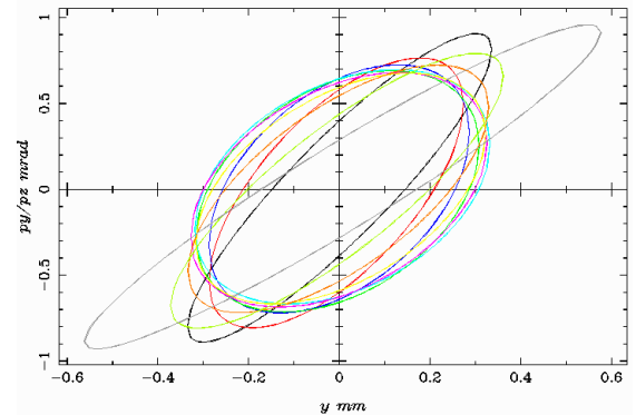
Figure 6: Ellipse of longitudinal bunch slice in y phase space giving 2.0 \pi mrad mm emittance at s=2.15 m.
