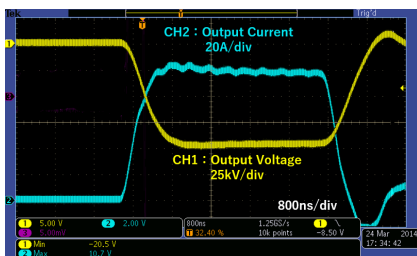
Figure 3: Output waveform of a direct-type klystron modulator.
