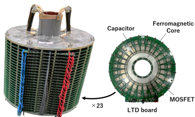
Figure 8: Picture of a LTD-type kicker power supply.
