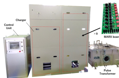
Figure 6: Picture of a MARX-type klystron modulator.
