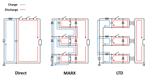
Figure 1: Three types of main circuits.
