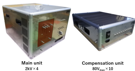
Figure 12: Picture of a MARX-type klystron modulator with droop compensation unit.
