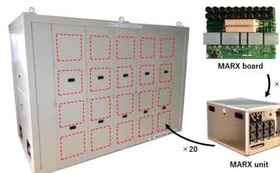
Figure 15: Picture of a MARX-type klystron modulator with PWM droop compensation.
