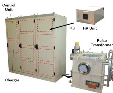
Figure 2: Picture of a direct-type klystron modulator.
