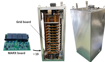
Figure 4: Picture of a MARX-type magnetron modulator.
