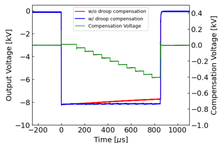
Figure 13: Output waveform of a MARX-type klystron modulator with droop compensation unit.
