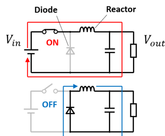
Figure 14: Schematic of a buck converter.
