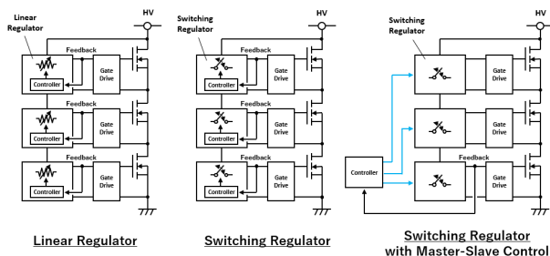
Figure 17: Three types of self-power feeding circuits.
