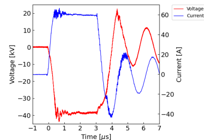
Figure 5: Output waveform of a MARX-type magnetron modulator.
