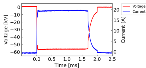
Figure 16: Output waveform of a MARX-type klystron modulator with PWM droop compensation.
