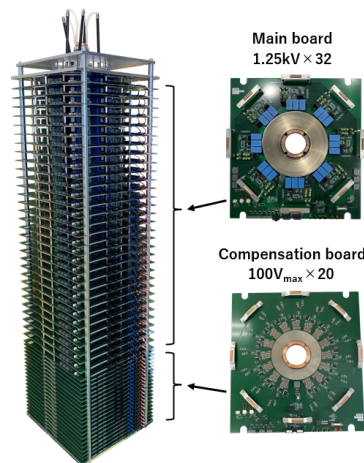
Figure 10: Picture of a LTD-type kicker power supply with droop compensation board.
