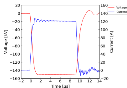
Figure 7: Output waveform of a MARX-type klystron modulator.
