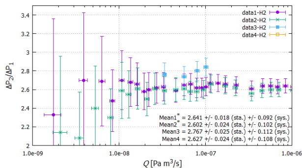
(a) Results of hydrogen introduction test.
