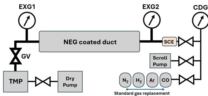
(a) Schematic diagram of the test equipment
