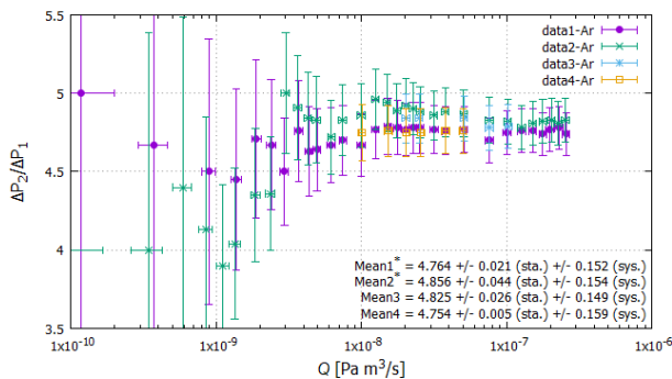
Figure 6: Result of Ar introduction test and pressure ratio for each experimental condition.
